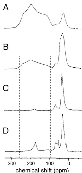
Fig. 2. ^{13}\text{C} NMR powder spectra of samples of ^{13}\text{C} -leucine-labeled bacteriorhodopsin (bR) [43]. The carbonyl carbon resonances are centered on 175 ppm and the aliphatic resonances are in the region 20 ppm–80 ppm. A. Hydrated native purple membrane at 3 °C. B. Reconstituted bR-containing DMPC bilayer vesicles at 3 °C. C. Same as in “B.” except at 30 °C. D. Same as in “C.” where the spectrum was obtained with a Hahn echo sequence. The vertical dashed lines mark the discontinuities of the rigid lattice carbonyl carbon chemical shift powder pattern. Fig. 2 is reprinted with permission from the American Chemical Society, copyright 1985 [43].
