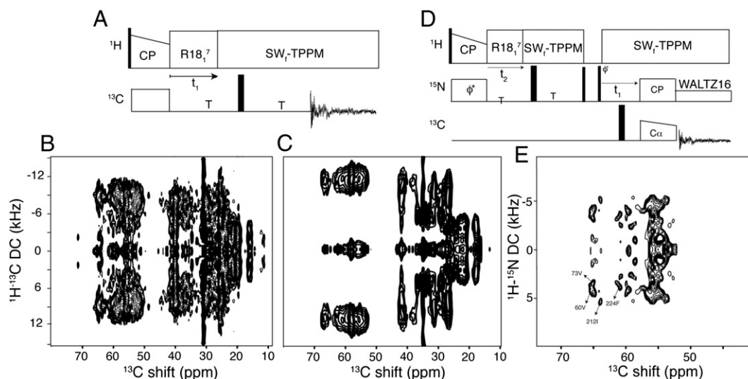
Fig. 12. Two- and three-dimensional separated local field (SLF) NMR spectra obtained from a uniformly ^{13}\text{C} and ^{15}\text{N} labeled sample of CXCR1 in DMPC bilayers. A. Pulse scheme used for recording the two-dimensional SLF data. B. ^1\text{H} - ^{13}\text{C} DC/ ^{13}\text{C} CS two-dimensional SLF correlation obtained at 30^\circ\text{C} . C. Same as B except at 10^\circ\text{C} . D. Pulse sequence for three-dimensional SLF NMR with ^{15}\text{N} editing and ^{13}\text{C} detection. Thin and wide solid lines represent the 90^\circ and 180^\circ pulses, respectively. ( \phi^* ) represents the phase sensitive data acquisition under States mode. E. Two-dimensional SLF plane from the three-dimensional spectrum correlating ^{13}\text{C} shifts with ^1\text{H} - ^{15}\text{N} DC obtained at 120.1 ppm ^{15}\text{N} shift. Cross peaks with single site resolution are marked with residue numbers.
