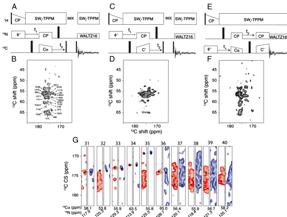
Fig. 11. Pulse sequences and spectra relevant to the three-dimensional correlation spectroscopy used to make sequential resonance assignments. A. and B. NCACO. C. and D. NCOCA. E. and F. CANCO. Thin and wide solid lines represent the 90^\circ and 180^\circ pulses, respectively. B., D. and F. are ^{13}\text{C}/^{13}\text{CO} two-dimensional planes obtained at 120.1 ppm ^{15}\text{N} chemical shift. The three-dimensional data were collected from a uniformly ^{13}\text{C} and ^{15}\text{N} labeled sample of CXCR1 in DMPC bilayers at 30^\circ\text{C} . G. Strip plot for residues 31–40 with nitrogen and carbon chemical shifts given below. Assigned residues are marked in the two-dimensional plane (D) obtained from NCACO three-dimensional data. Data were collected with 4–5 ms ^{13}\text{C} and 6 ms ^{15}\text{N} isotropic shift evolution in indirect dimensions, and 12 ms during direct ^{13}\text{C} acquisition under heteronuclear decoupling. Equal numbers of data points in the indirect dimension were linearly predicted. 0.2 ppm line broadening was used in the direct dimension during data processing. Each of the three-dimensional data sets was collected with approximately 1000 scans.
