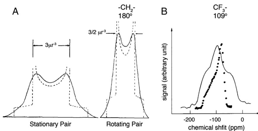
Fig. 1. Motional averaging of powder patterns. A. ^1\text{H} – ^1\text{H} dipole–dipole powder patterns (Pake doublets) for two proximate ^1\text{H} nuclei that are stationary (left) or undergoing 180^\circ internal motion (right) [49]. B. ^{19}\text{F} chemical shift powder patterns of silver trifluoroacetate at 107 K (dark dots) and 40 K (solid line). The spectra are characteristic of rotating (107 K) and rigid (40 K) \text{CF}_3 groups [55].
