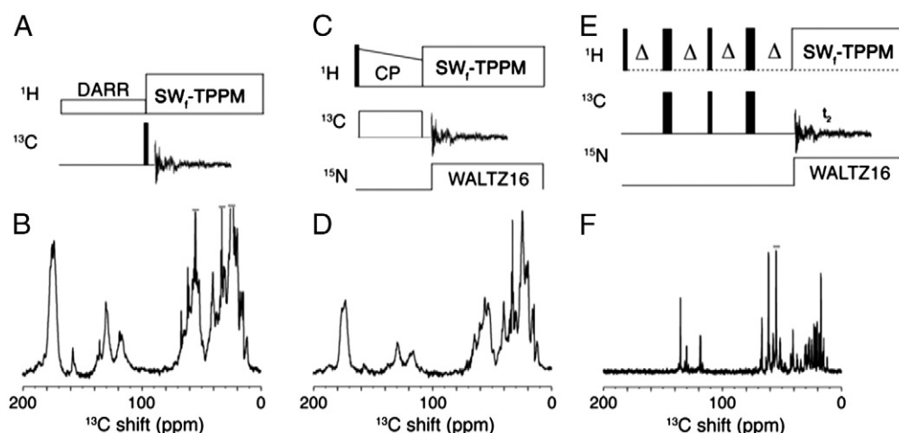
Fig. 8. One-dimensional pulse sequences for ^1\text{H} to ^{13}\text{C} cross polarization (CP) and experimental results obtained from a uniformly ^{13}\text{C} and ^{15}\text{N} labeled sample of CXCR1 in DMPC phospholipid bilayers. A. and B. Nuclear Overhauser polarization transfer in MAS (NOP-MAS). C. and D. Hartmann–Hahn CP MAS. E. and F. Insensitive nuclei enhanced by polarization transfer (INEPT) MAS. B., D., and F. ^1\text{H} decoupled ^{13}\text{C} -detected one-dimensional spectra NMR obtained using the pulse schemes shown directly above. Experiments were carried out with 10 kHz MAS at 30 °C. Continuous wave radio frequency irradiation with amplitude less than 10 kHz was applied for 1 s for NOP-MAS. 100 kHz RF with swept frequency two-pulse phase modulation (SWH-TPPM) was applied for ^1\text{H} decoupling. 62 kHz RF irradiation was applied on the ^{13}\text{C} nuclei in all experiments. Cross-polarization transfer in CP-MAS was obtained with 1 ms mixing and for t periods in INEPT. One-dimensional data from CP and NOP were recorded with 100 scans each and 1000 scans for INEPT.
