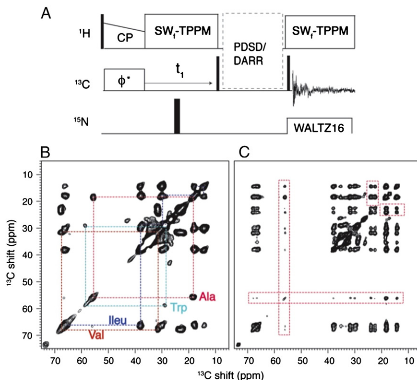
Fig. 9. ^{13}\text{C}/^{13}\text{C} homonuclear correlation spectra of the trans-membrane domain of Vpu in DMPC bilayers obtained at 15 °C. The sample consisted of 2 mg of labeled protein in 10 mg DMPC. A. Pulse scheme to record spin-exchange data. Thin and thick solid lines represent 90^\circ and 180^\circ pulses, respectively. B. and C. Two-dimensional NMR spectra correlating aliphatic carbons obtained for 50 ms and 500 ms PDSD mixing with 11 kHz MAS, respectively. The dashed lines in B. correlate ^{13}\text{C} shifts within a residue type. The rectangular boxes in C. represent the cross peaks that resulted from long mixing. They are potentially from inter-residue or inter-helical contacts between residues. ( \phi^* ) represents the phase sensitive data acquisition using States mode. The spectra were obtained from 5 ms and 15 ms chemical shift evolution in indirect and direct acquisition dimensions, respectively.
