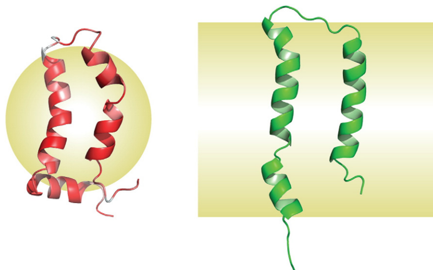
Fig. 16. Comparison of the structures of full-length 63-residue p7 in micelles and bilayers. A. Structure in DHPC micelles. B. Structure in DMPC bilayers. The structure in micelles is drastically distorted from that in bilayers. The cartoon micelle suggests that the distortion is caused by the requirement of the N-terminal helix to be in a hydrophobic environment.
